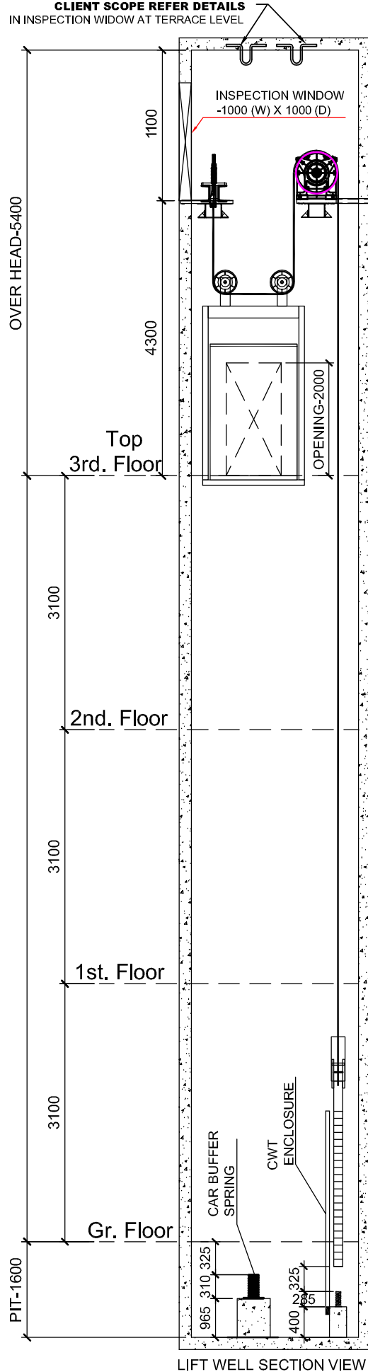
LIFT WELL SECTION VIEW
